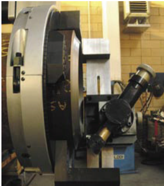
Crossbar allows rigidity and precision when making bevel on pipes with wall thickness over 50 mm (2"), also for inside bevel and ID boring up to 100 mm depth.
